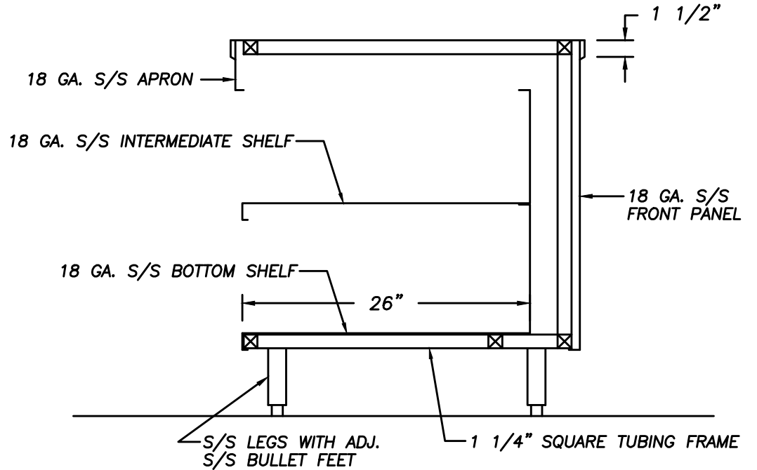
SECTION 1"=1'-0"
