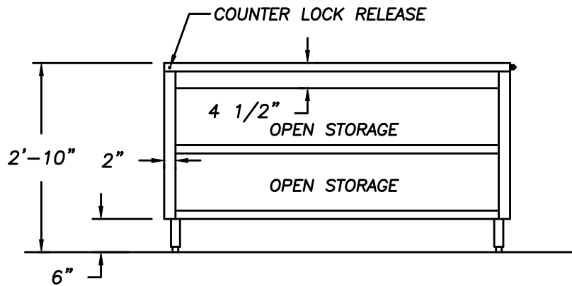
REAR ELEVATION 1/2"=1'-0"
