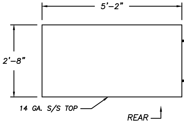
PLAN VIEW 1/2"=1'-0"
